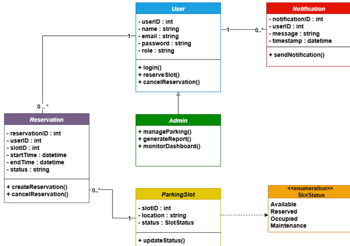
SMART PARKING SYSTEM FOR UNIVERSITY CAMPUS UML CLASS DIAGRAM
